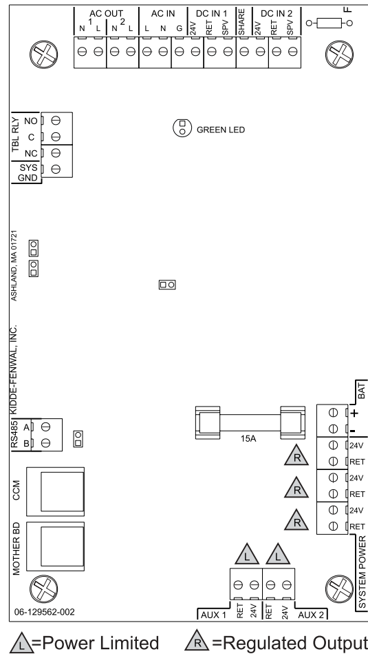
Figure 1. Power Supply Wiring Diagram
