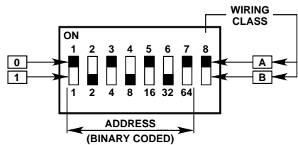
SWITCH DIAGRAM ABOVE SHOWS AN ADDRESS OF 0101010 = 42 CLASS "A" WIRING
