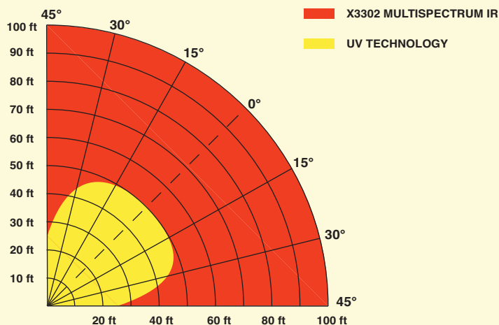
DETECTOR HORIZONTAL FIELD OF VIEW TO HYDROGEN FIRE (24 INCH PLUME, WITH 100 GRAMS/MIN FLOW RATE)
